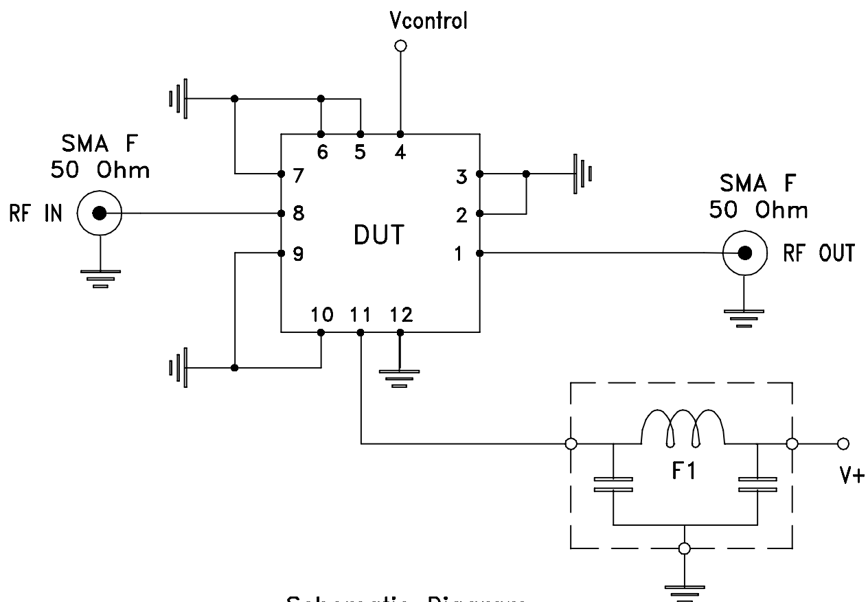
Schematic Diagram
