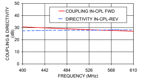
SYBD-28-62HP+ COUPLING & DIRECTIVITY
