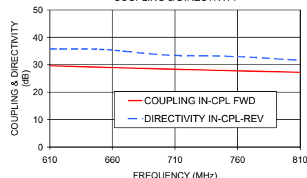
SYBD-28-82HP+ COUPLING & DIRECTIVITY
