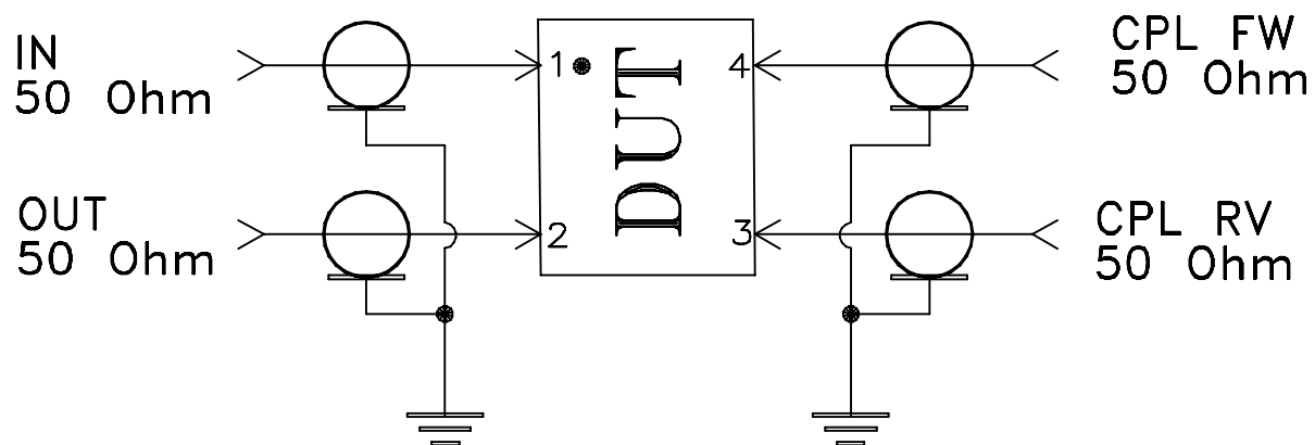
Schematic Diagram
