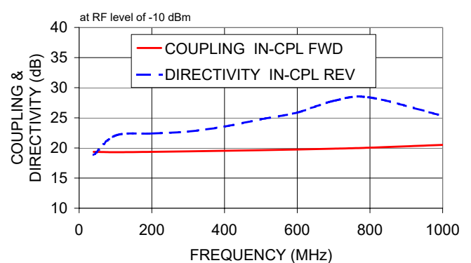
SYDC-20-13HP+ COUPLING & DIRECTIVITY
