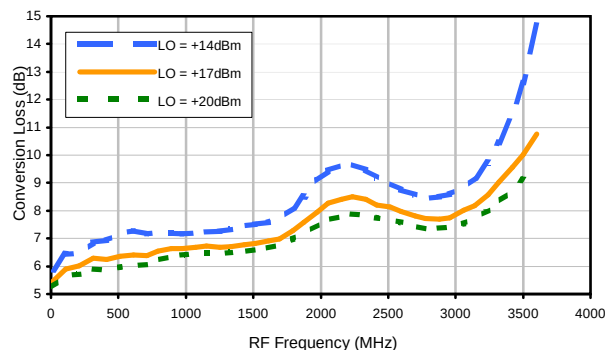
Conversion Loss vs. LO @ RF=1900.1MHz
