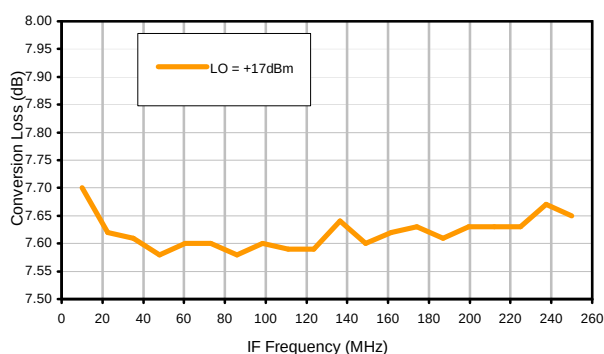
Conversion Loss vs. IF @ RF=2400.1MHz
