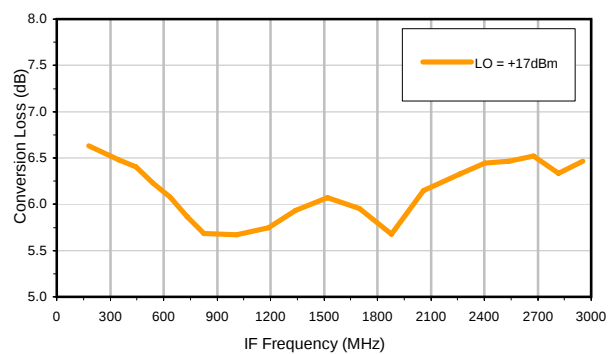
Conversion Loss vs. IF @ RF=3810.1 MHz
