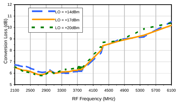
Conversion Loss vs. LO @ RF=3770.1 MHz
