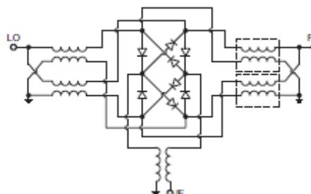
Electrical Schematic
