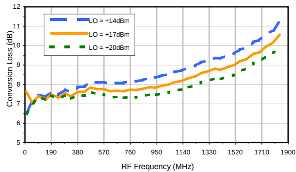
Conversion Loss vs. LO @ RF=945 MHz
