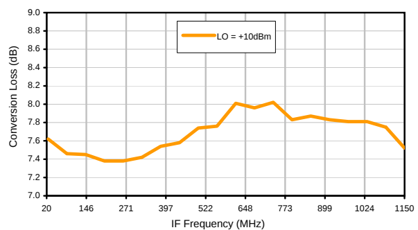
Conversion Loss vs. IF @ RF=1785.1MHz
