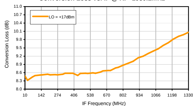
Conversion Loss vs. IF @ RF=1930.1MHz
