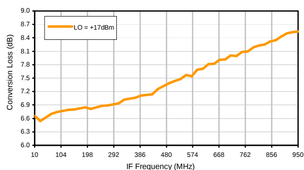
Conversion Loss vs. IF @ RF=970.1MHz
