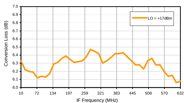
Conversion Loss vs. IF @ RF=652.1MHz
