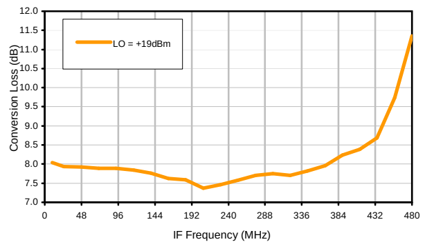
Conversion Loss vs. IF @ RF=910.1MHz
