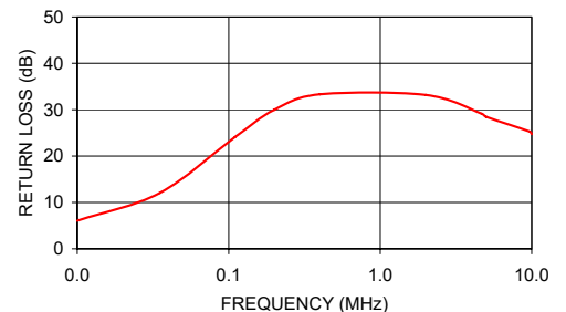
T-626-X65 INPUT RETURN LOSS
