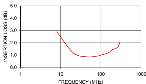
T1-1H INSERTION LOSS
