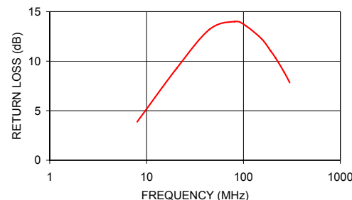
T1-1H INPUT RETURN LOSS
