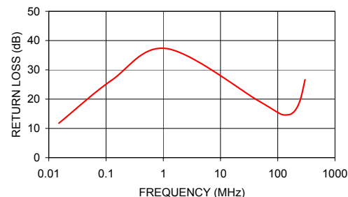
T1-6T-KK81 INPUT RETURN LOSS
