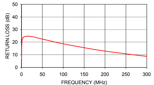
T1.5-1 INPUT RETURN LOSS
