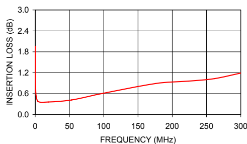
T1.5-1 INSERTION LOSS
