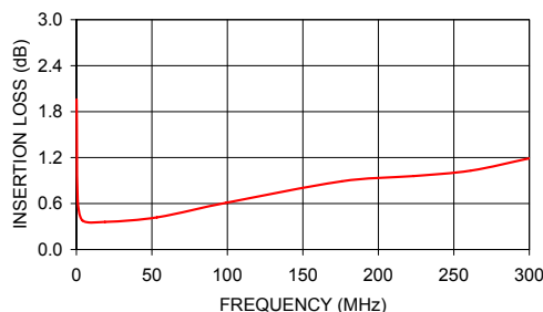
T1.5-1-KK81 INSERTION LOSS
