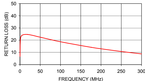
T1.5-1-KK81 INPUT RETURN LOSS
