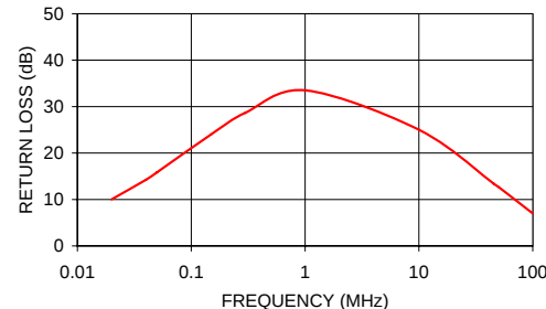
T1.5-6 INPUT RETURN LOSS
