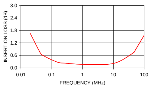
T1.5-6 INSERTION LOSS
