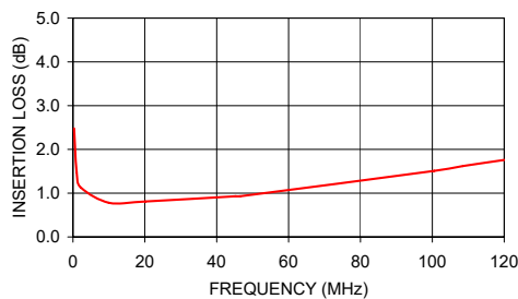
T16-1-X65 INSERTION LOSS
