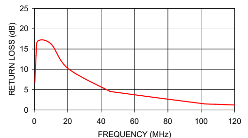
T16-1-X65 INPUT RETURN LOSS
