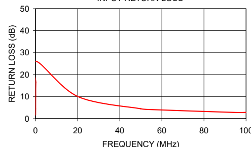
T2.5-6T-X65 INPUT RETURN LOSS
