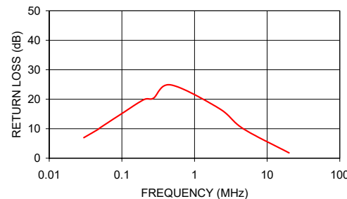
T36-1-X65 INPUT RETURN LOSS
