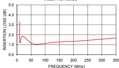
T4-1H INSERTION LOSS
