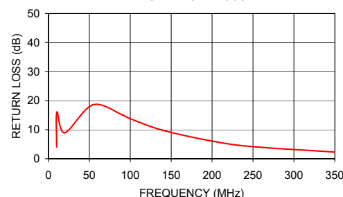
T4-1H INPUT RETURN LOSS
