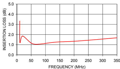
T4-1H-KK81 INSERTION LOSS
