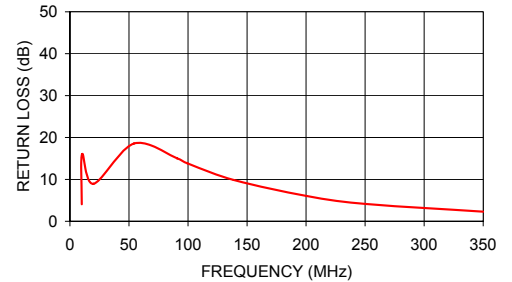
T4-1H-KK81 INPUT RETURN LOSS
