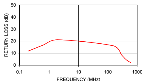
T4-2 INPUT RETURN LOSS
