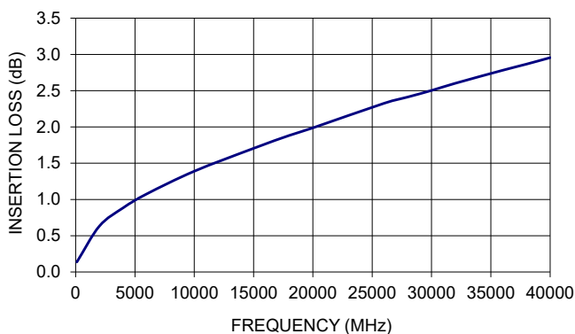
T40-3FT-KMKM+ INSERTION LOSS
