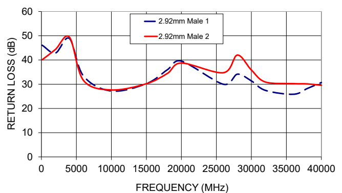
T40-3FT-KMKM+ RETURN LOSS
