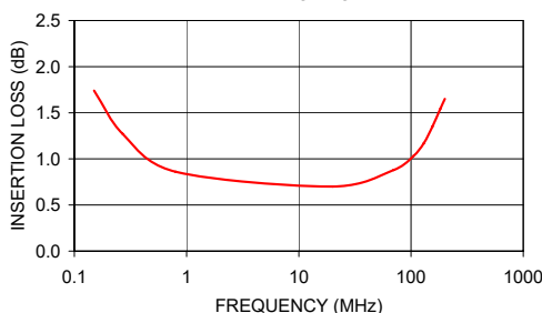
T9-1-X65 INSERTION LOSS
