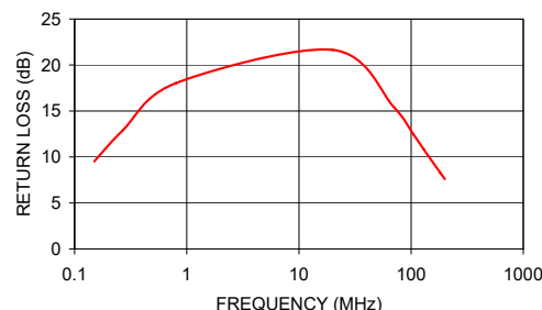
T9-1-X65 INPUT RETURN LOSS
