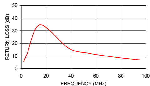
T9-1H-X65 INPUT RETURN LOSS
