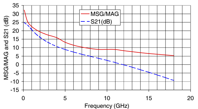
MAXIMUM STABLE GAIN (MSG)/MAXIMUM AVAILABLE GAIN (MAG) vs. FREQUENCY V_{DS}=4V & I_{DS}=15mA
