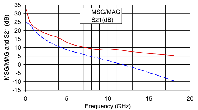
MAXIMUM STABLE GAIN (MSG)/MAXIMUM AVAILABLE GAIN (MAG) vs. FREQUENCY V_{DS}=3V & I_{DS}=15mA
