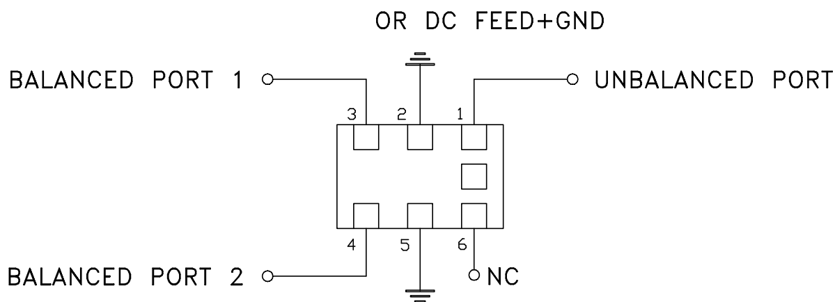
Schematic Diagram
