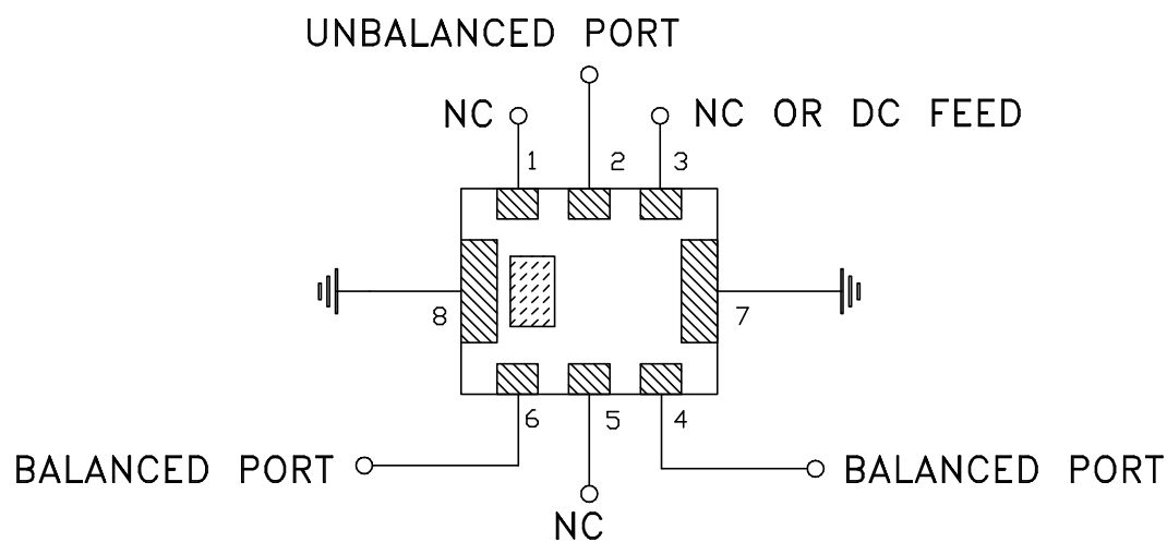
Schematic Diagram
