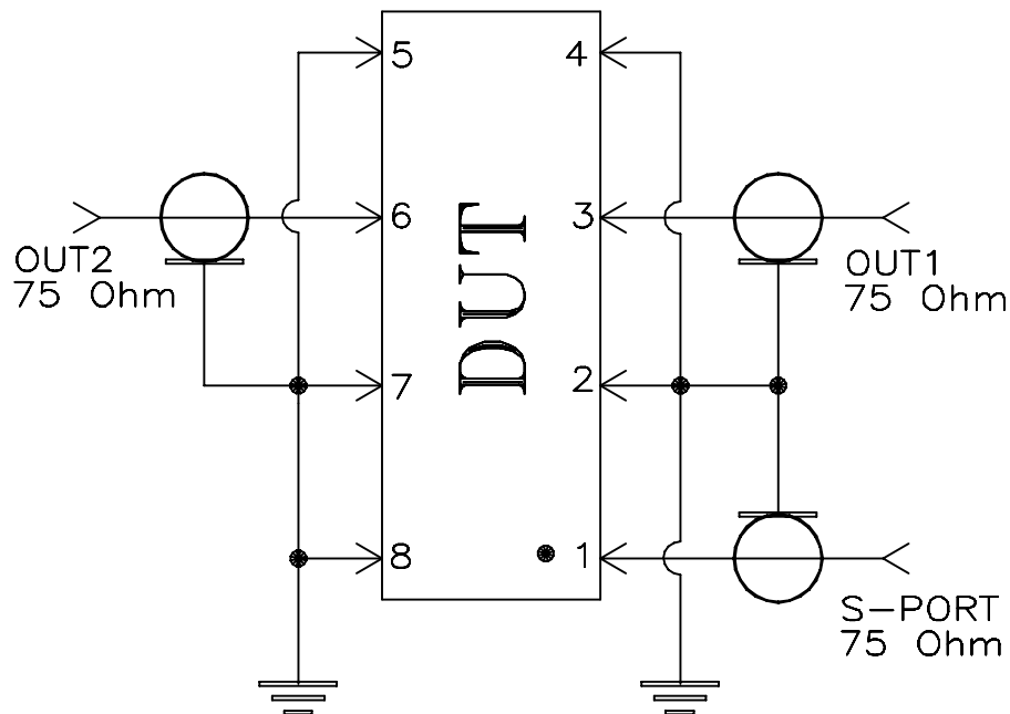
Schematic Diagram
