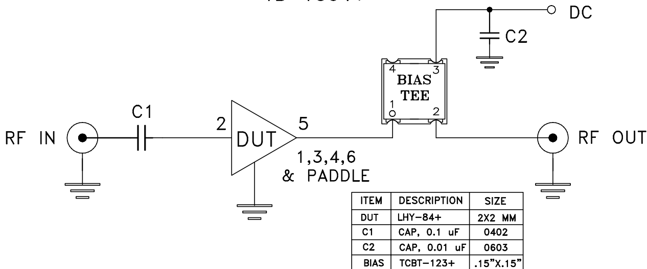
Schematic Diagram
