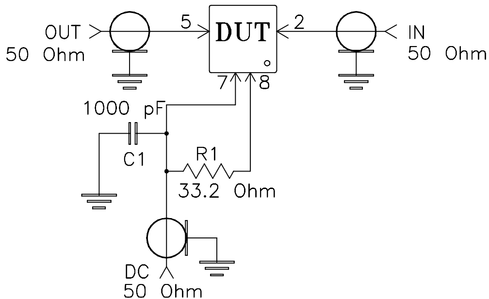
Schematic Diagram
