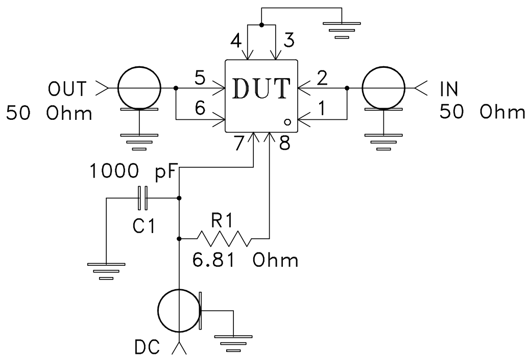
Schematic Diagram
