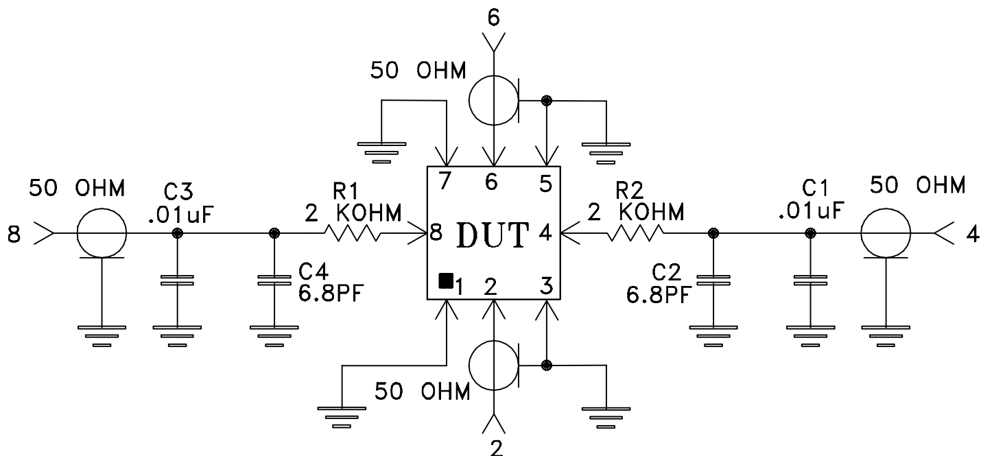
Schematic Diagram
