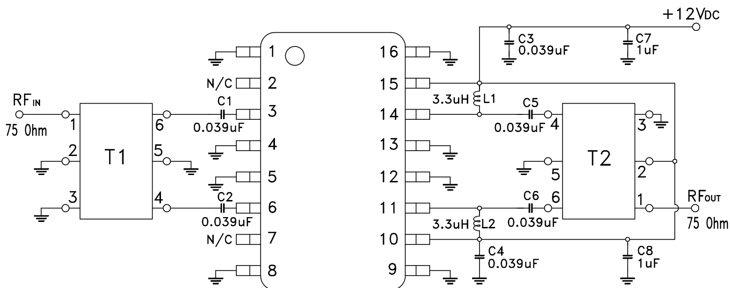
Schematic Diagram
