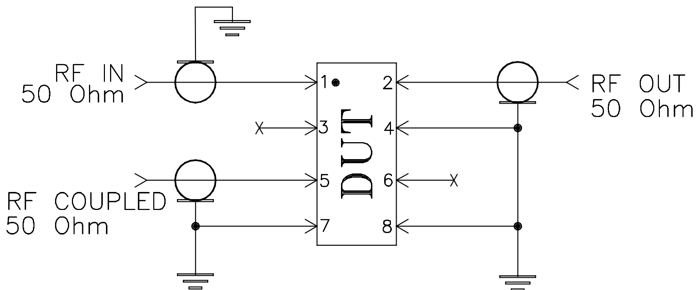
Schematic Diagram
