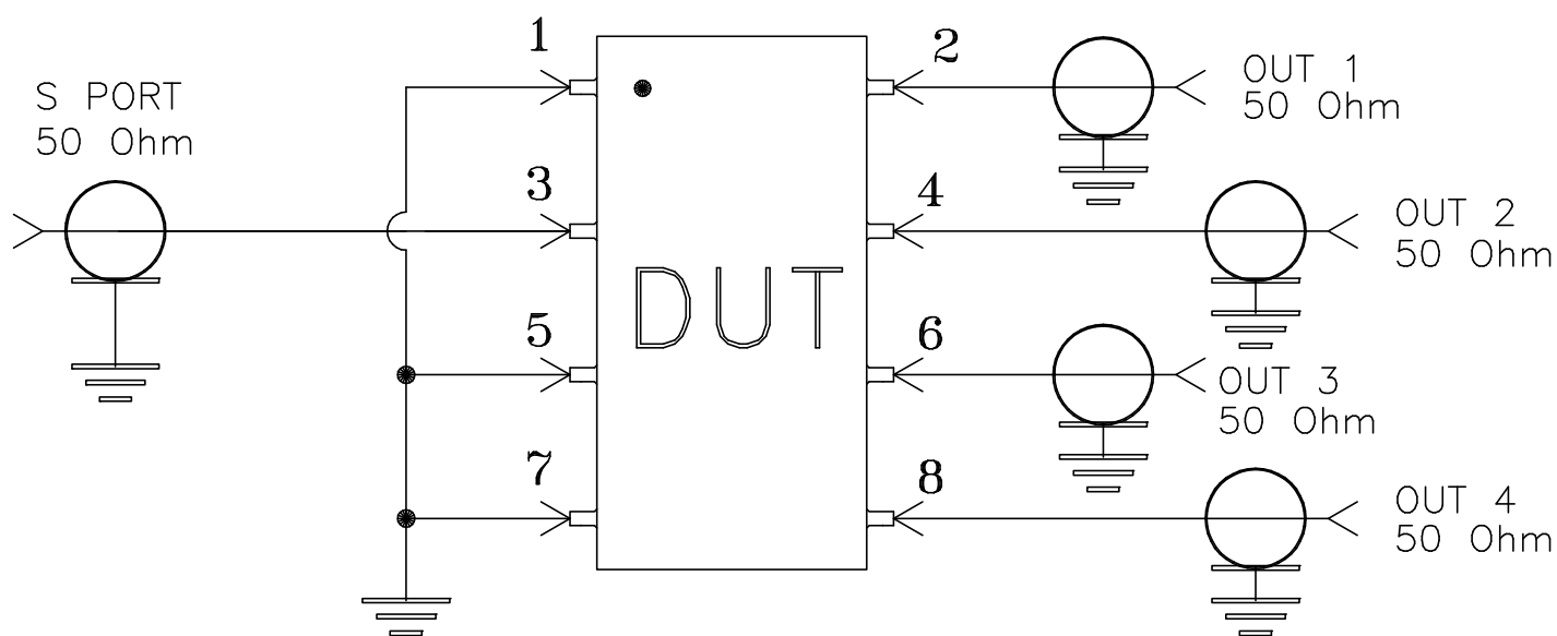
Schematic Diagram
