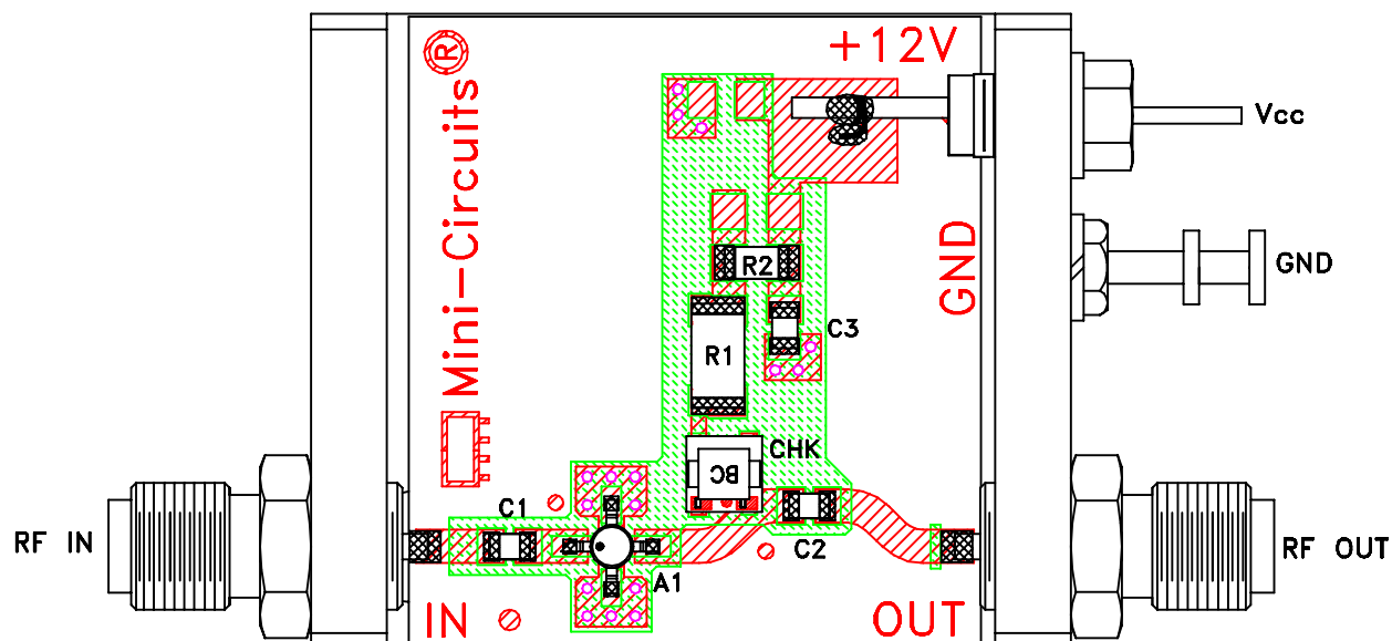
TB-408-50+
