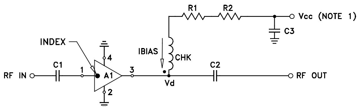
TB-408-50+
