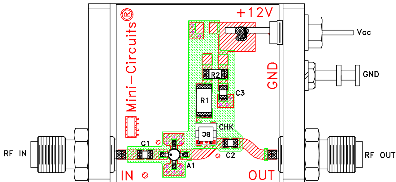
TB-414-6A+
