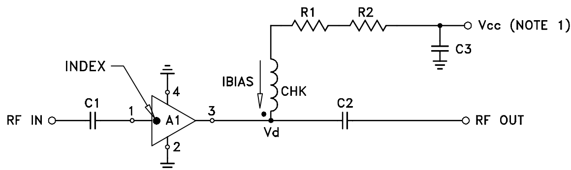
TB-414-6A+
