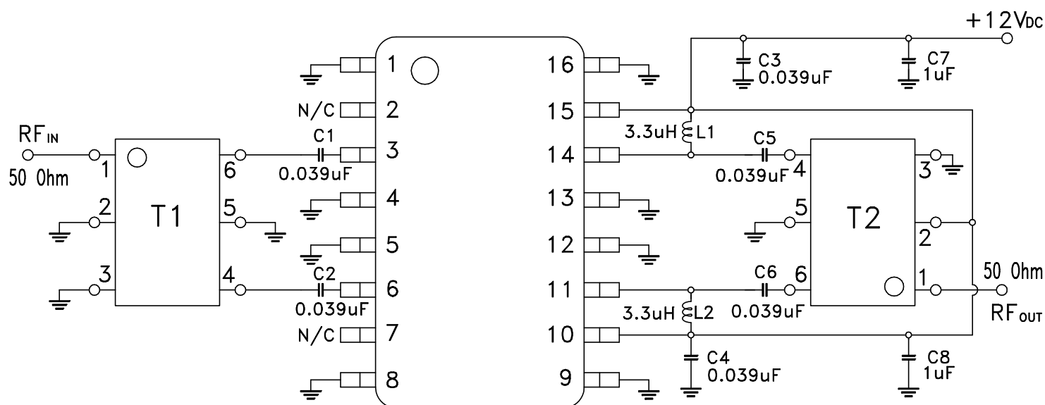
Schematic Diagram
