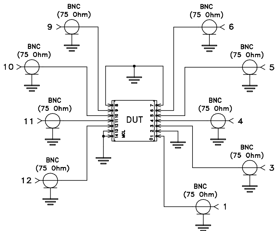
Schematic Diagram
