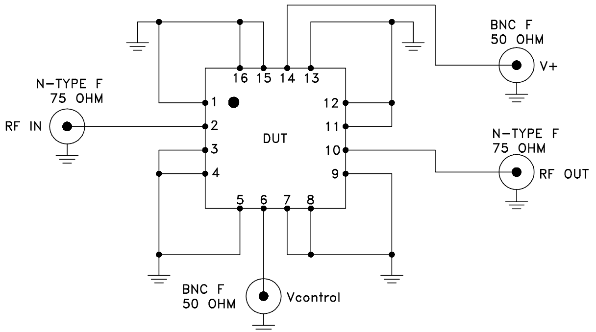
Schematic Diagram
