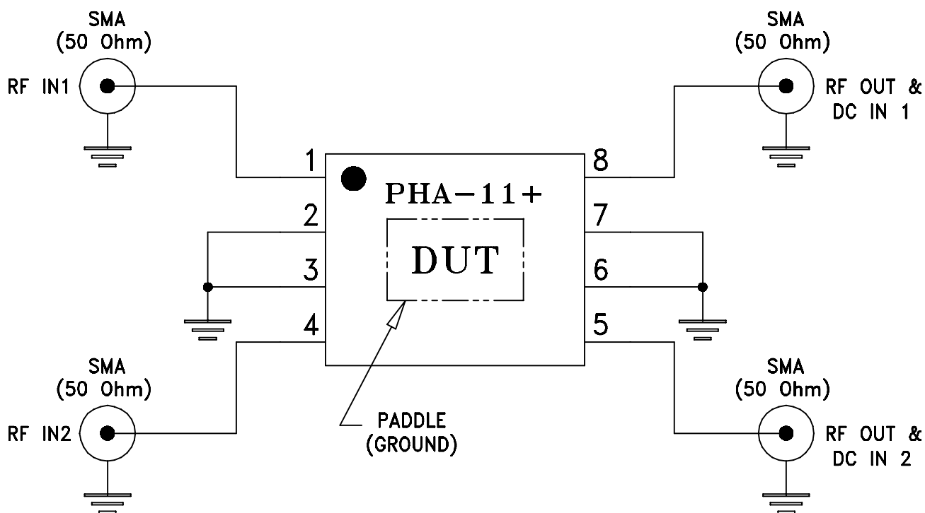
Schematic Diagram
