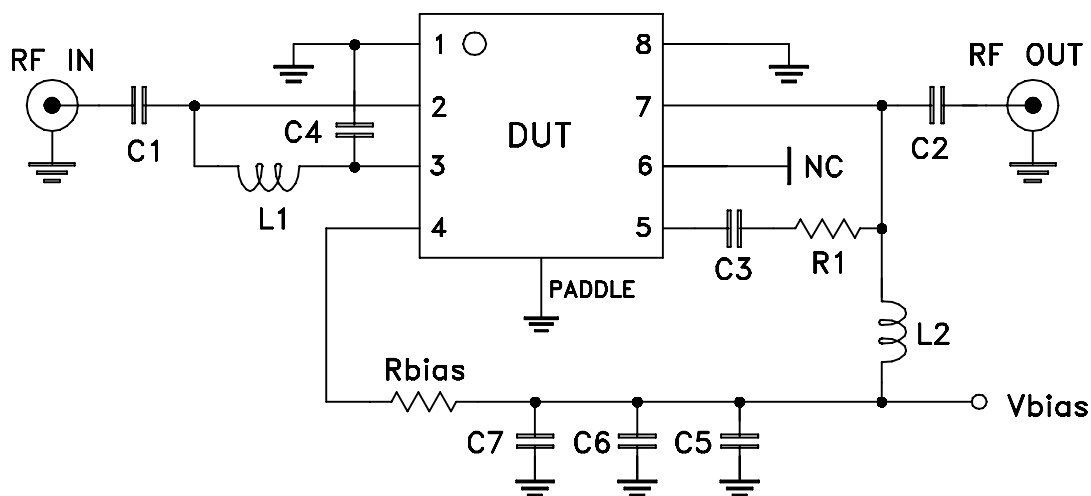
ITEM DESCRIPTION C1, C6 CAP, 9.1pF C2, C4 CAP, 100pF C3 CAP, 5.6pF C5, C7 CAP, 0.1uF R1 RES, 267 Ohm Rbias RES, 750 Ohm L1 IND, 6.8nH L2 IND, 15nH DUT PMA2-162LN+
