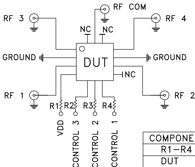
Schematic Diagram
