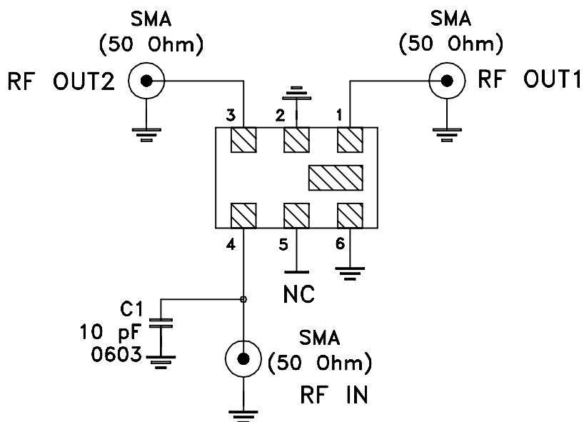
Schematic Diagram
