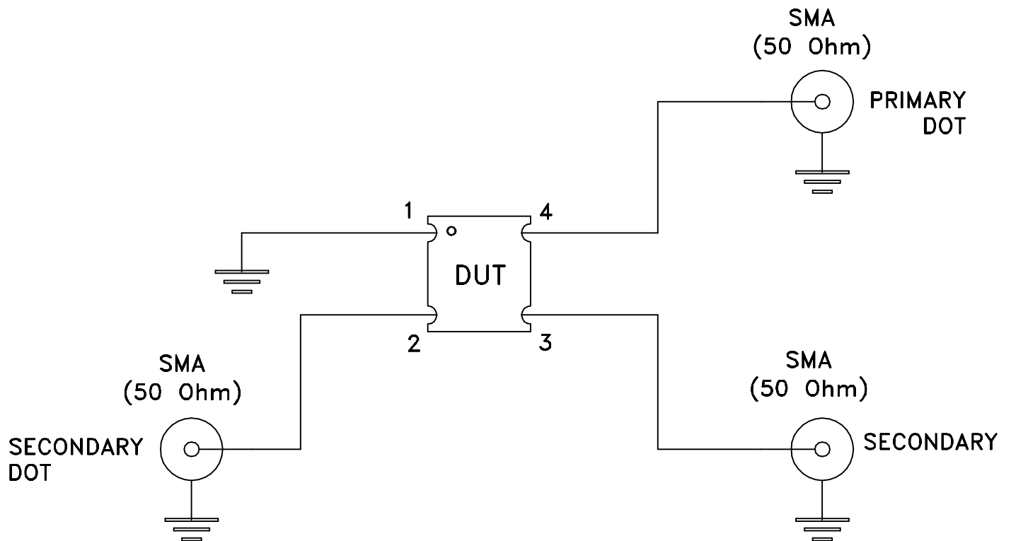
Schematic Diagram
