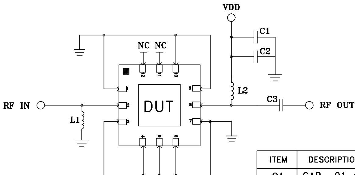
Schematic Diagram
